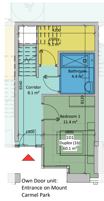
① AT-1D1 - Lower Level 1:100
