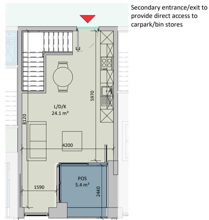
① AT-1D1 - Lower Level 1:100
