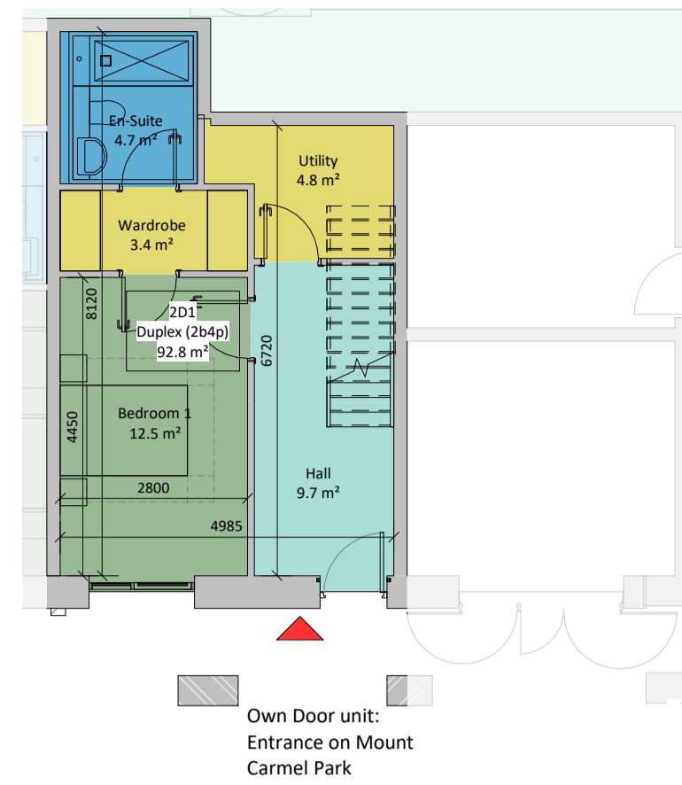
③ AT-2D1 - Lower Level 1:100
