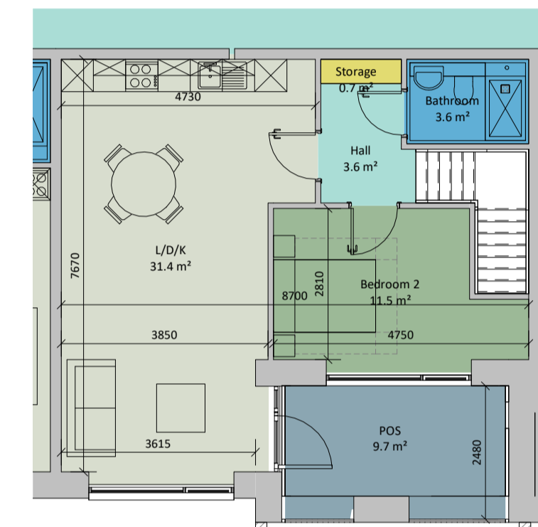
⑤ AT-2D2 - Lower Level 1:100
